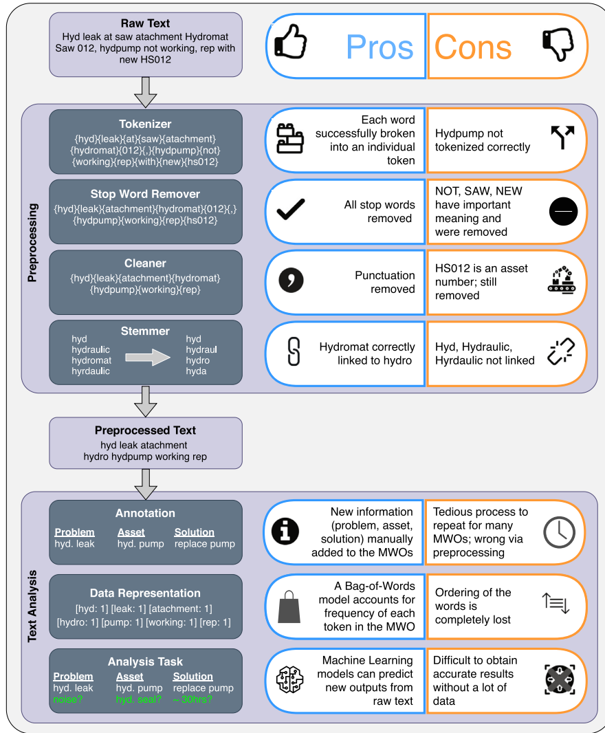
Fig. 1. A common NLP workflow for technical language text data. The left side of the figure illustrates the output of each step. The right side shows the pros and cons of each step when applied to technical text. This example is meant to be illustrative of real problems that can arise with NLP pipelines on technical text.
